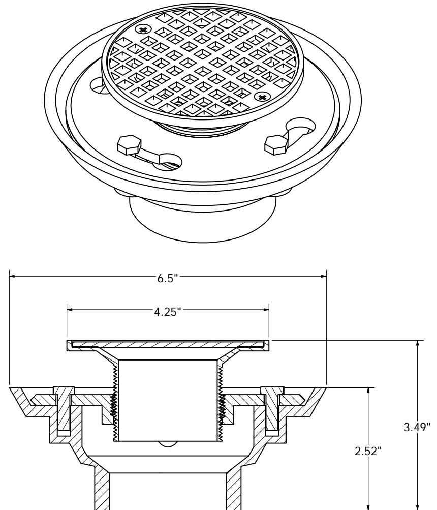
SECTION A-A SCALE 1
