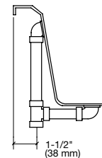
PLUMBING ROUGH-IN
