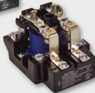
DPDT with auxiliary
