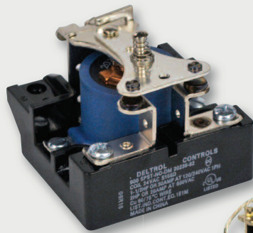
SPST-NO
