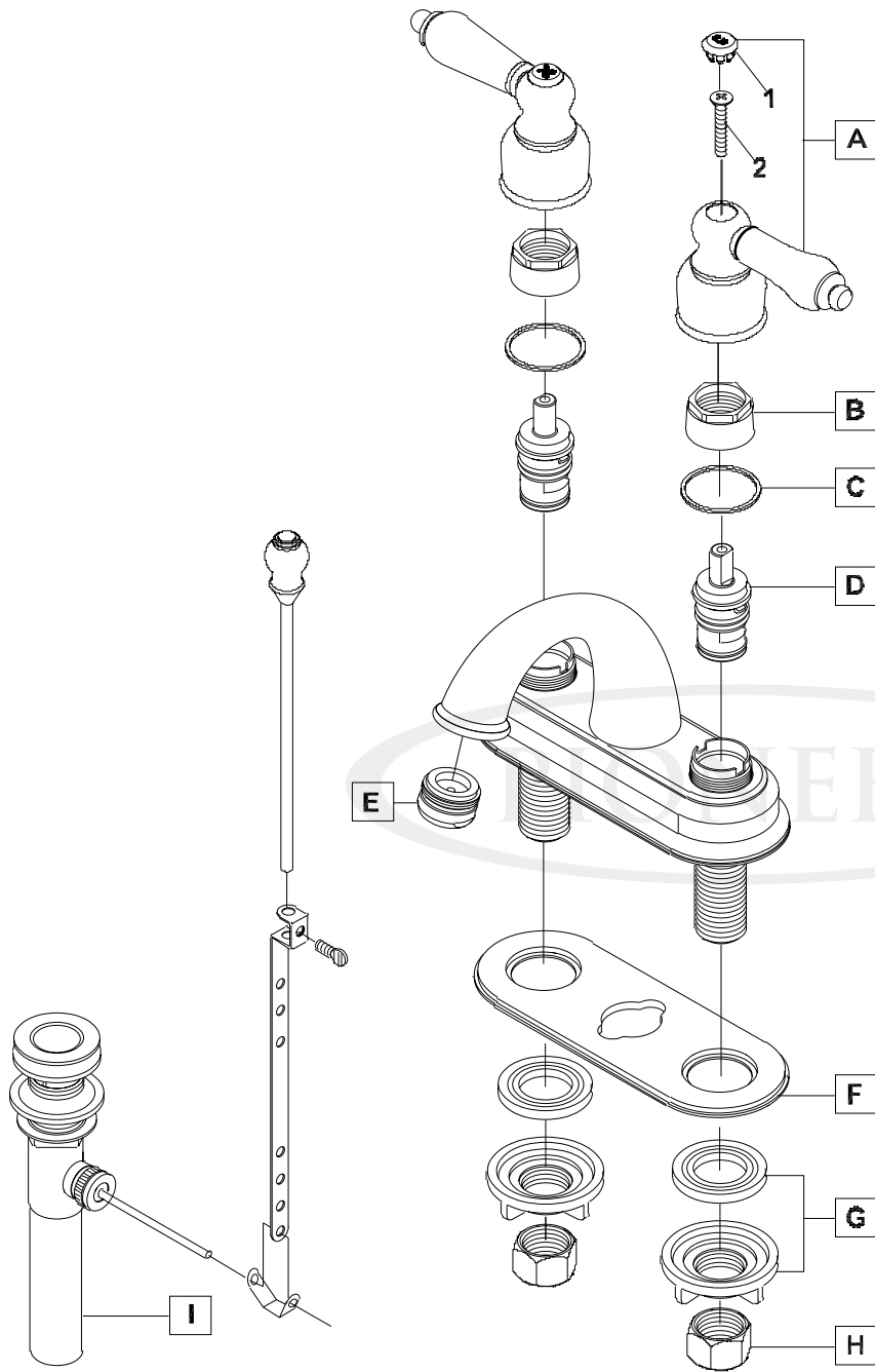
Product Diagram
