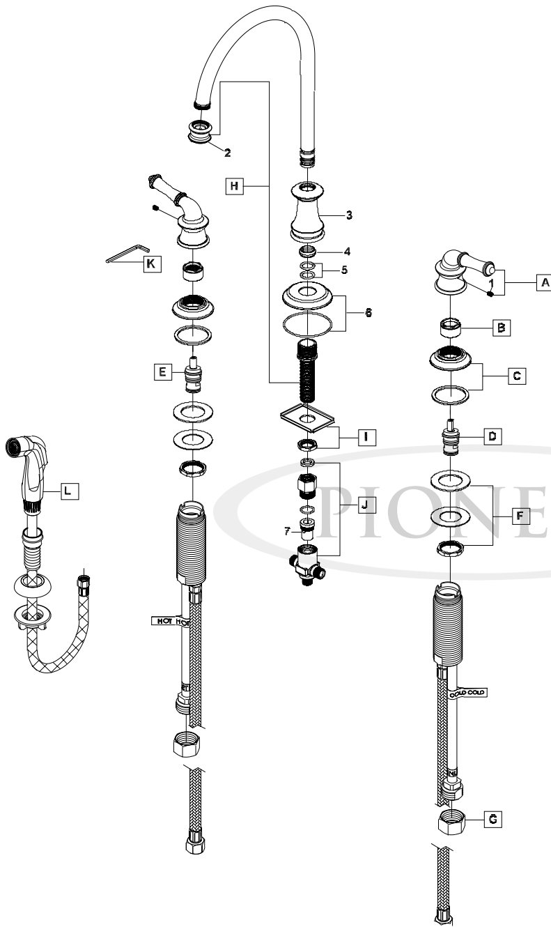
Product Diagram
