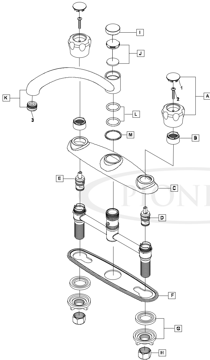
Product Diagram
