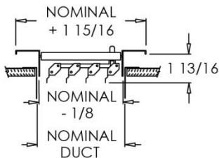
945 (Stamped Steel One Piece Frame)
