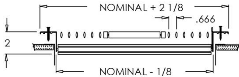
945-O (Extruded Aluminum Frame)
