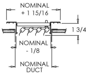
945 (Extruded Aluminum Frame)
