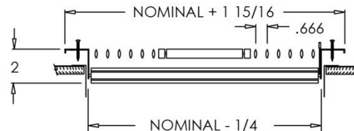
945 (Stamped Steel One Piece Frame)
