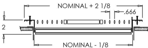
945 (Extruded Aluminum Frame)
