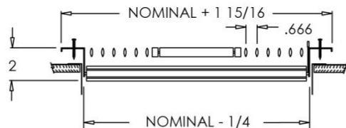
945-O (Stamped Steel One Piece Frame)
