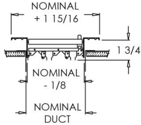
945-O (Extruded Aluminum Frame)
