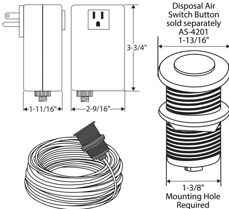
10' Air Tube & Mounting Shank ASB-4201
