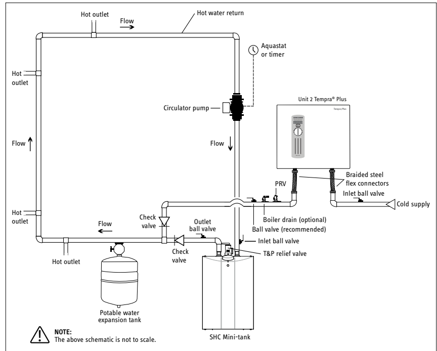
Tempra® and SHC Mini-Tank recirculation loop
