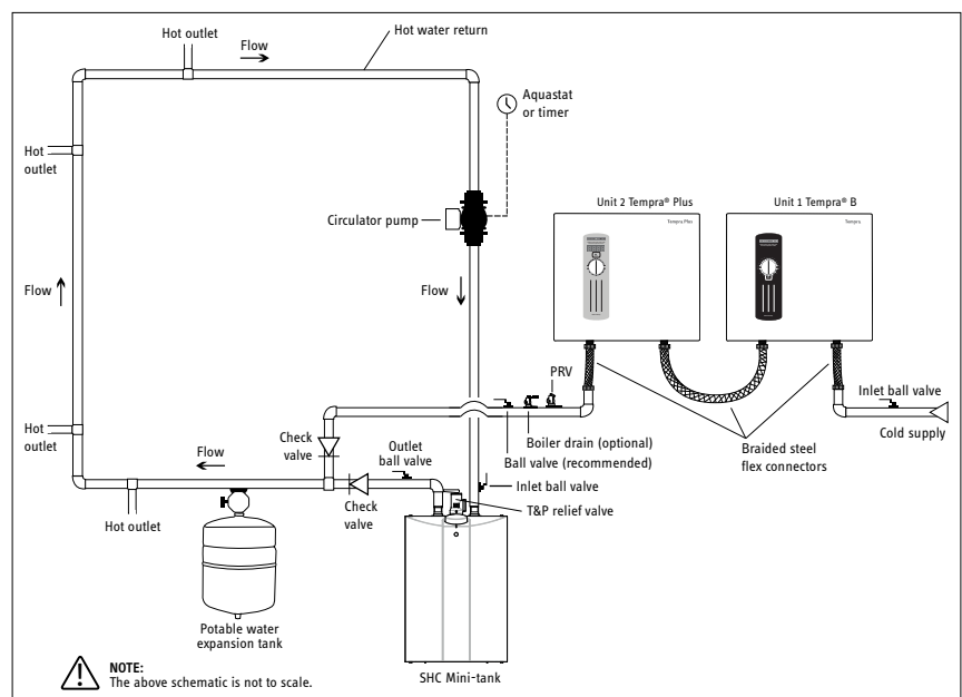
Tempra® and SHC Mini-Tank recirculation loop
