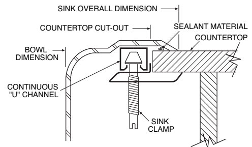
Lancelot® Double Bowl Kitchen Sink Model: 22395 (LDE- 33" x 22"- 4)
