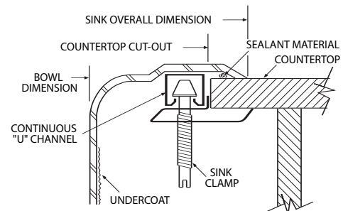
Installation Detail
