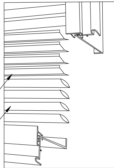
Detail View of Right Front Corner Blade Angle
