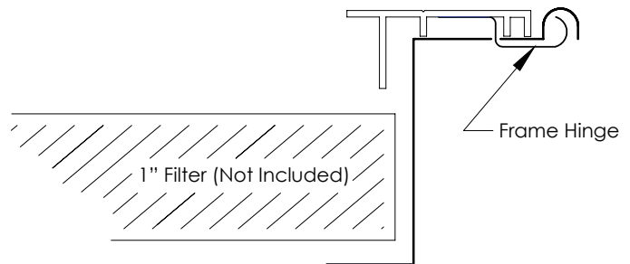
620FG1 Frame Detail
