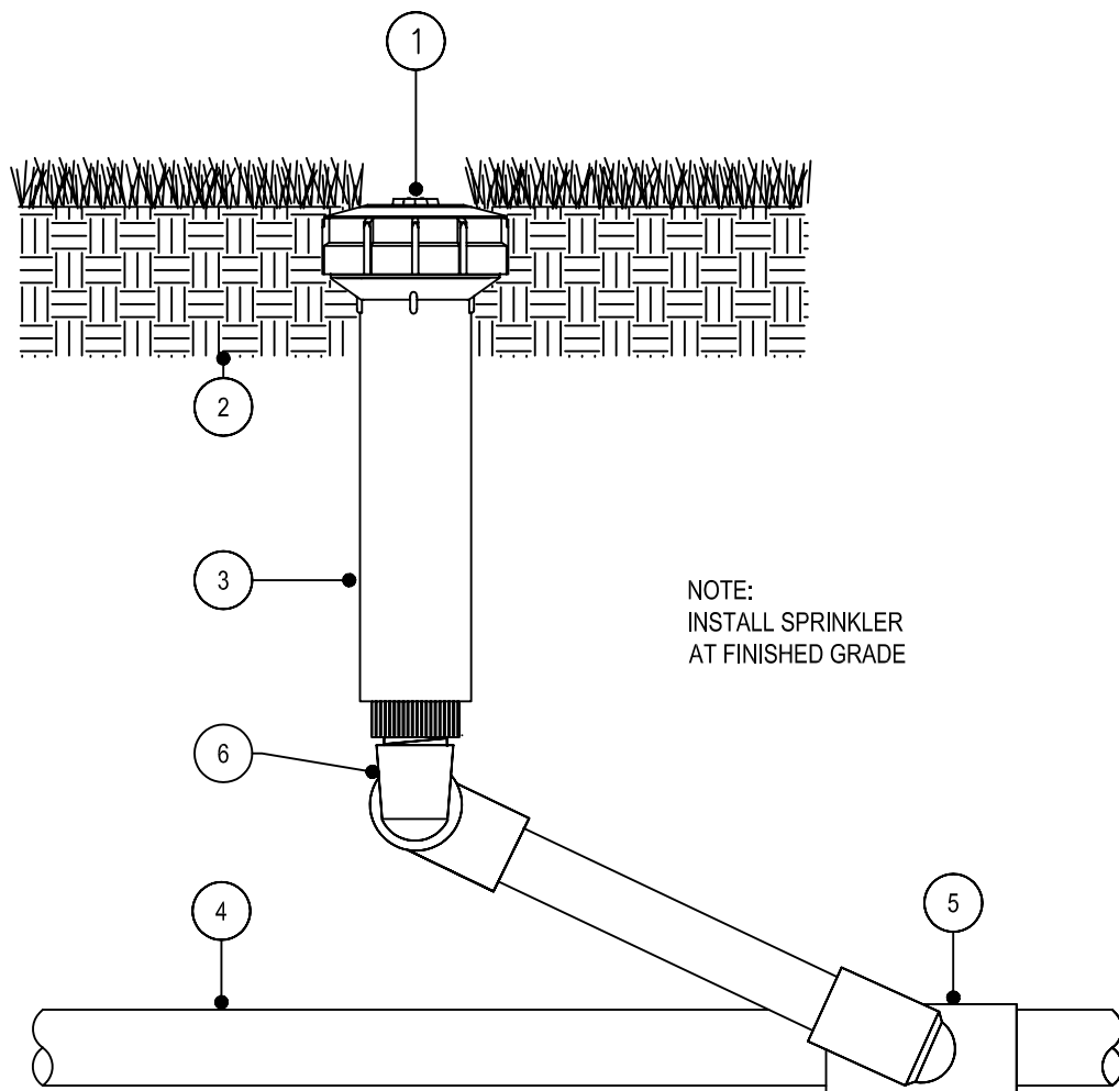
SECTION/ELEVATION NOT TO SCALE
