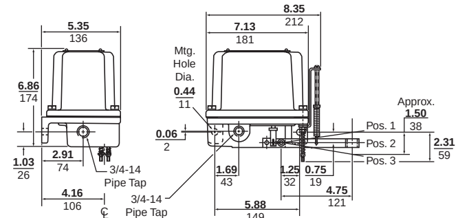
Figure 19: Type AR1/AW1 Dimensions
