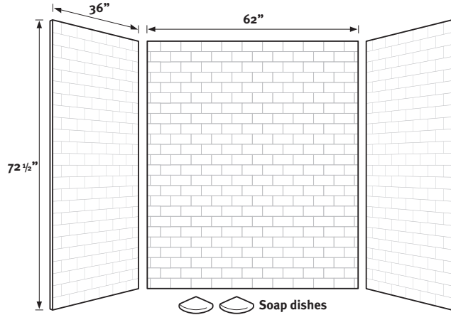
Designed to fit base areas 36" deep or smaller x 62" wide x 72-1/2" high or smaller (914 mm x 1575 mm x 1829 mm)
