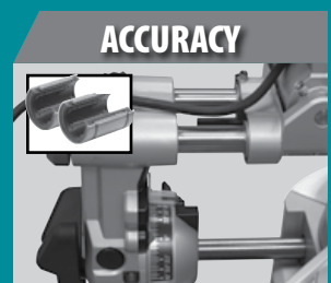
6 linear ball bearings and 4-steel rail sliding system deliver maintenance-free "dead-on" accurate cuts
