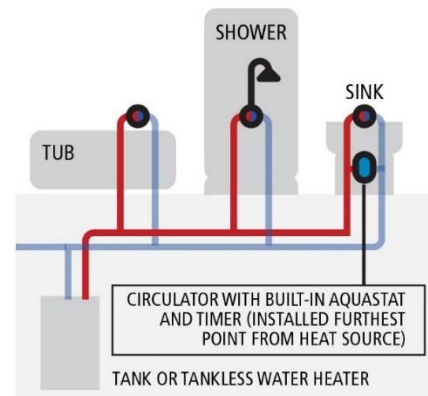
Installation Diagram with Timer
