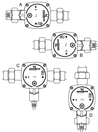
Fig. Power head positions
