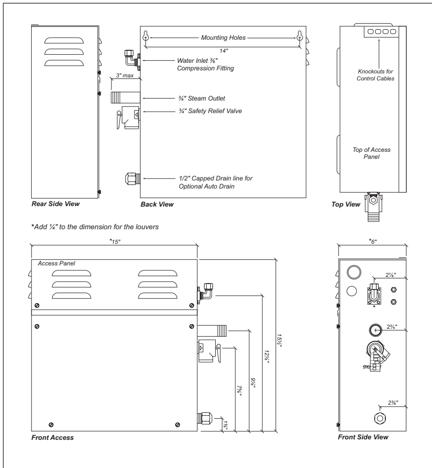
Steam Generator Specification Chart
