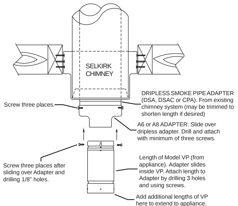
Fig. 1 ATTACHMENT OF VP ADAPTER TO EXISTING SELKIRK CHIMNEY INSTALLATION
