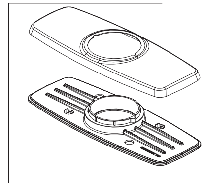
RP102244 ▲ (Escutcheon optional, included) Escutcheon with Gasket (3 Hole) Chapetón y Empaque (3 agujeros) Boîtier et Joint (3 trous)
