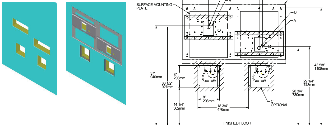
Figure 1 - Rough-in EDFPB(V)117C
