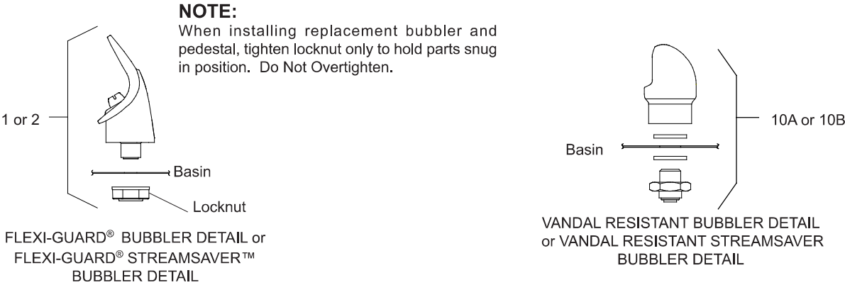
Figure 8 - Bubbler Details
