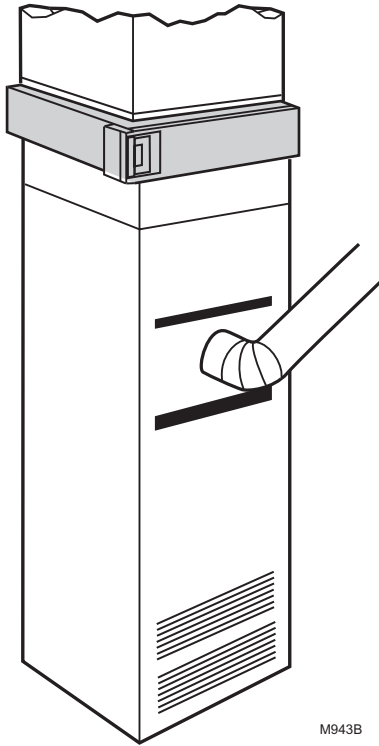
Fig. 5. Counterflow furnace, with Electronic Air Cleaner mounted horizontally in return duct or plenum just above furnace.
