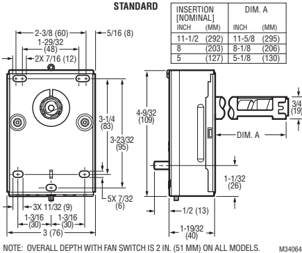
Fig. 6. L4064 Dimensions.
