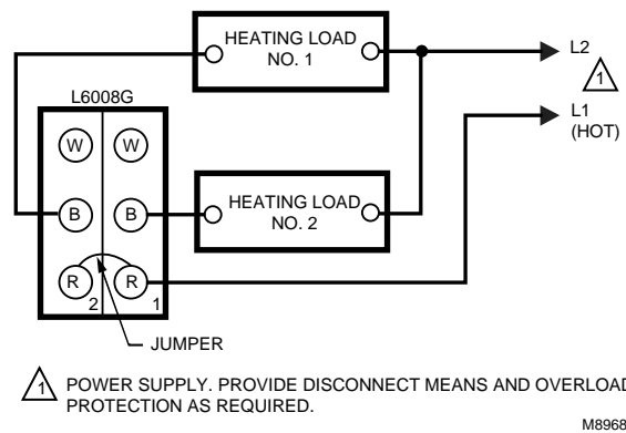
Fig. 28. Typical oil burner installation using L4008G.
