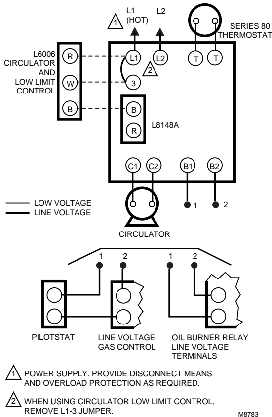
Fig. 25. Typical wiring hookup using L6006 or L6007 with L8148A.
