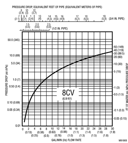
Fig. 2c. Flow characteristics of 8 Cv (6.9 kV) valve.
