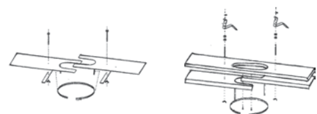
VSK Damper Sealing Kit
