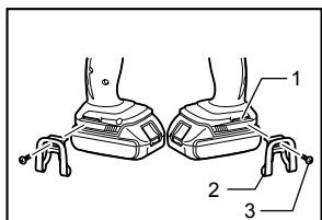
1. Groove 2. Hook 3. Screw
