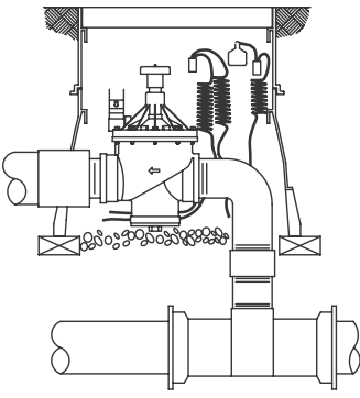
Heavy Duty 3" Remote Control Valve Globe Installation
