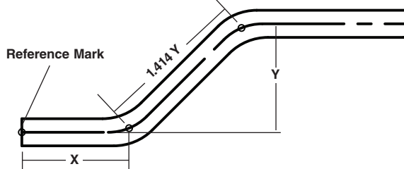
B – Bent Tube with Markings
