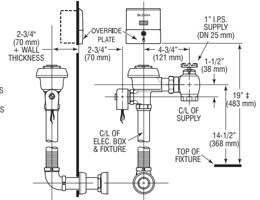
MODEL 140 ES-S
