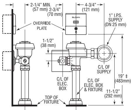
MODEL 152 ES-S
