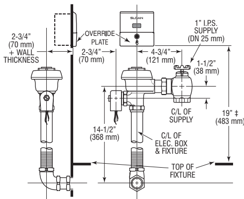
MODEL 152 ES-S
