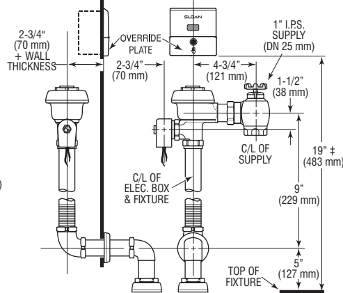
MODEL 153 ES-S
