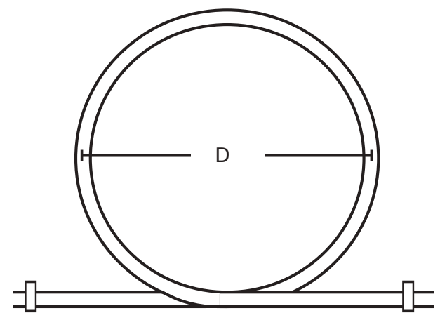
Figure 17.4 Coiled Loop Expansion
