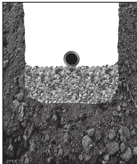
Trench in poor soil
