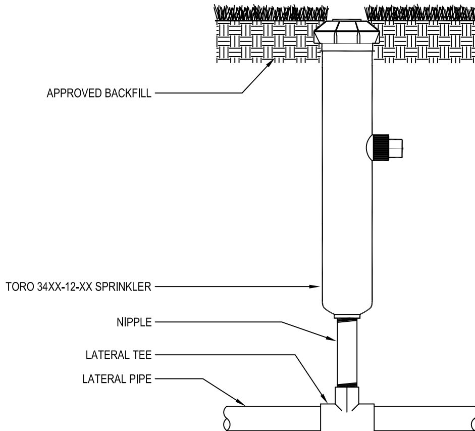
SECTION/ELEVATION NOT TO SCALE
